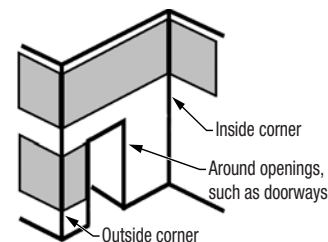
Figure 12. Re-squeegee to ensure good adhesion
