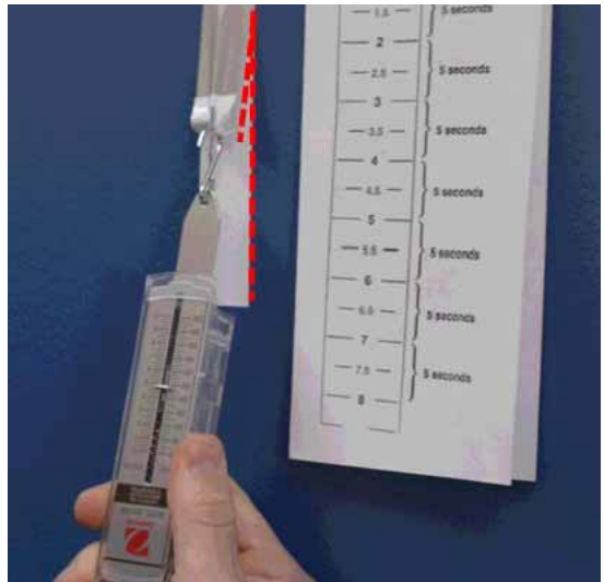
Figure 5. Adhesion test
